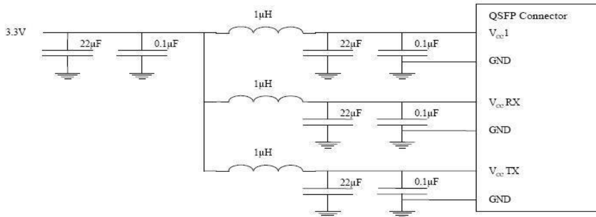
Figure3. Host Board Power Supply Filtering
