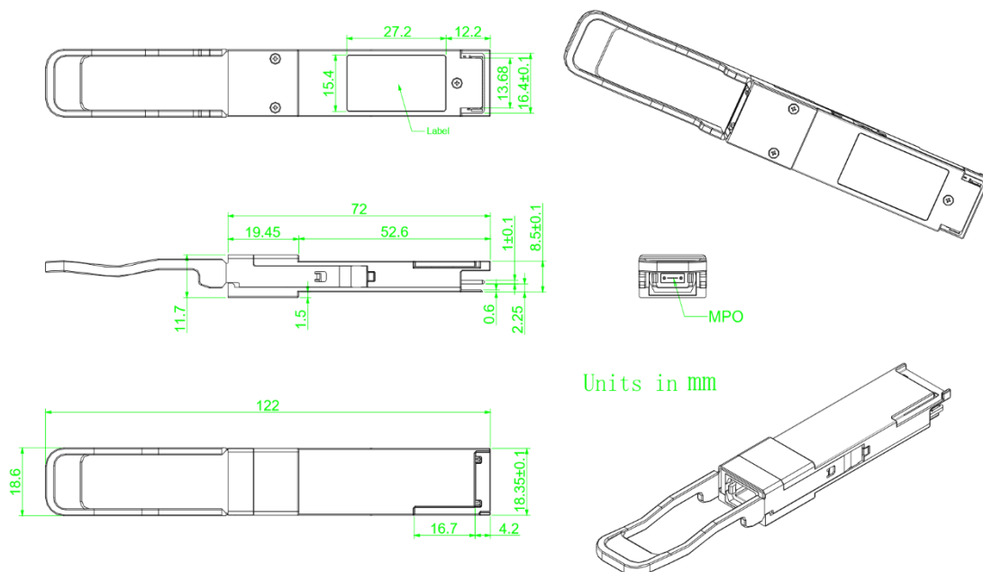
Figure10. Mechanical Specifications
